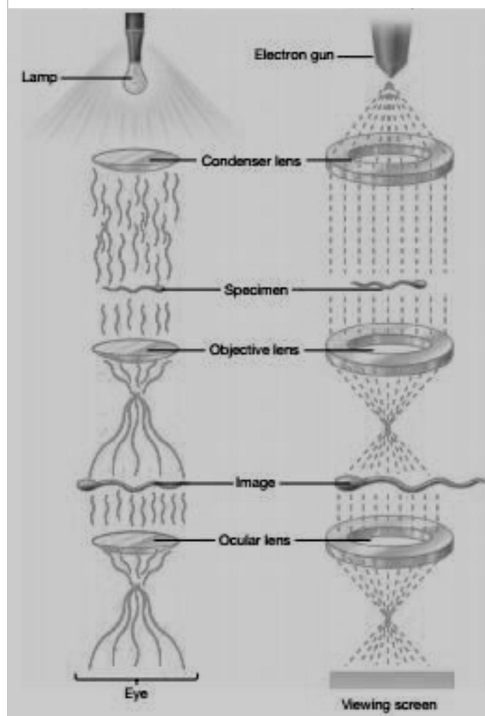
Figure 1 Label the diagram of electron microscope?
